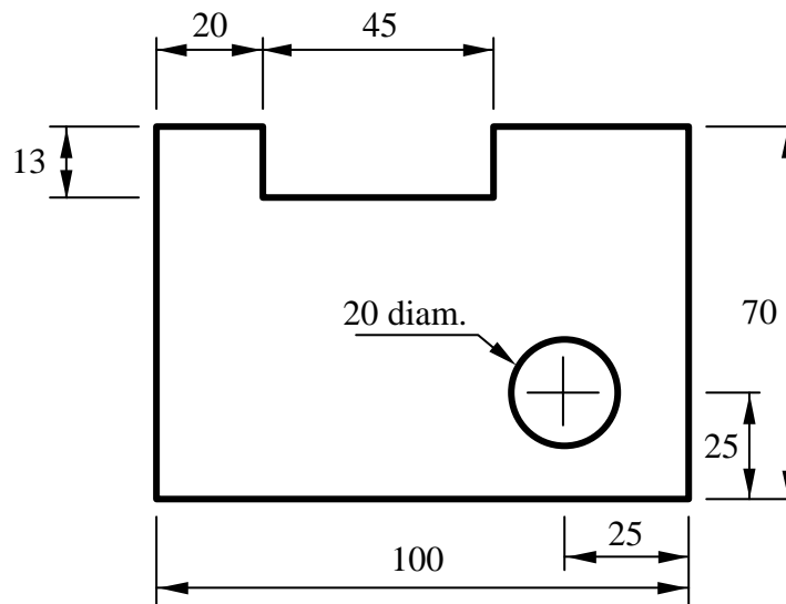
Figure 3-13. Plate to be constructed in Concept Analyst
