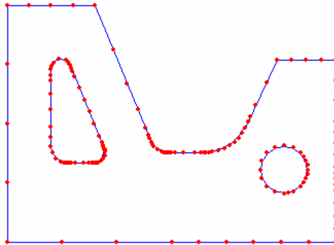
Figure 8-7 Final mesh from adaptive run starting from a coarse mesh
