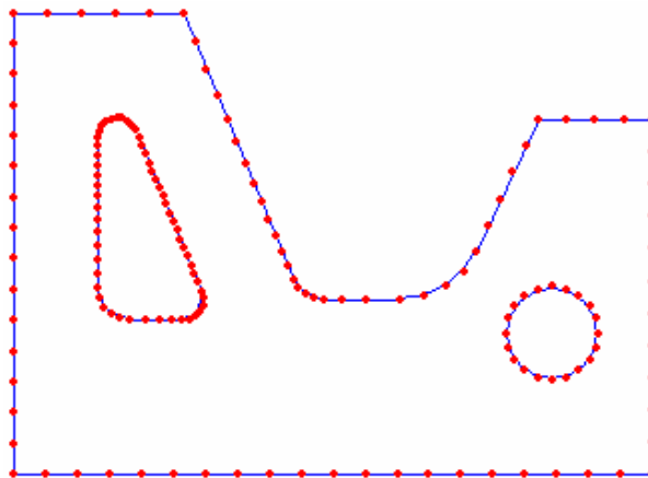
Figure 8-5 Fine mesh
