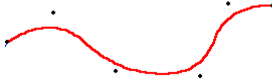
Figure 3-9. B-spline and its control points
