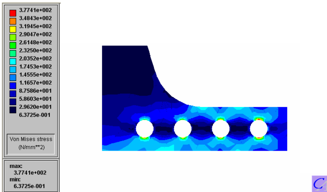
Figure 9-3. Contour plot of results
