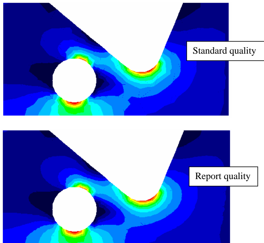
Figure 9-8. Comparison of standard and report quality contours
