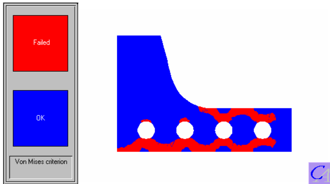
Figure 9-4. Failure criterion contour plot
