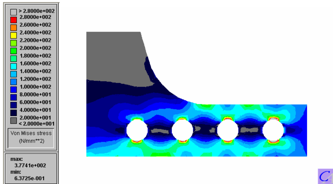
Figure 9-6 Contour plot with user-defined ranges
